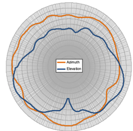
Q910 Antenna Patterns
