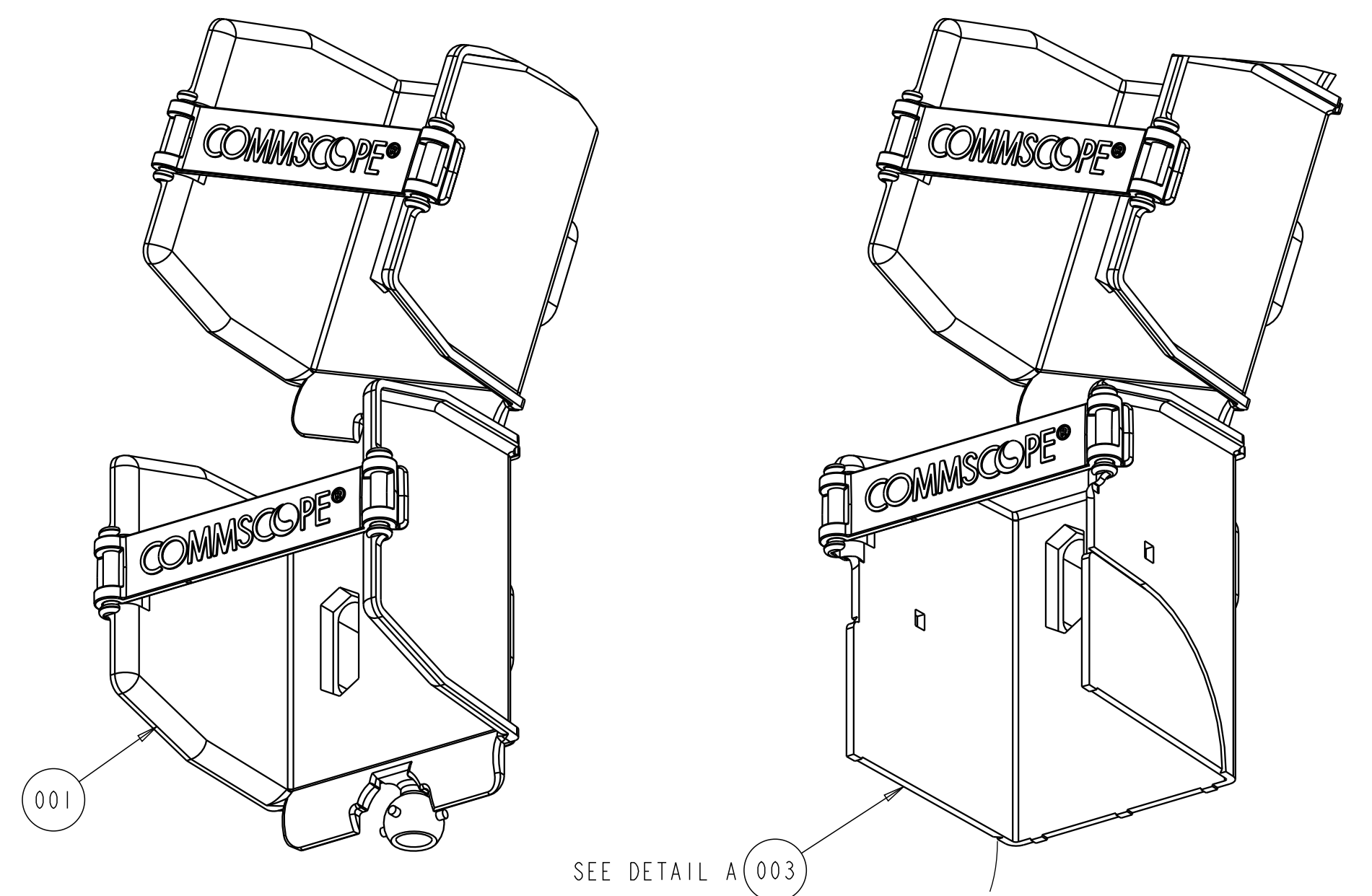
OPTION 1 2X2 TROUGH (USED IF CONNECTING TO FLEX VERTICAL TROUGH KIT)
