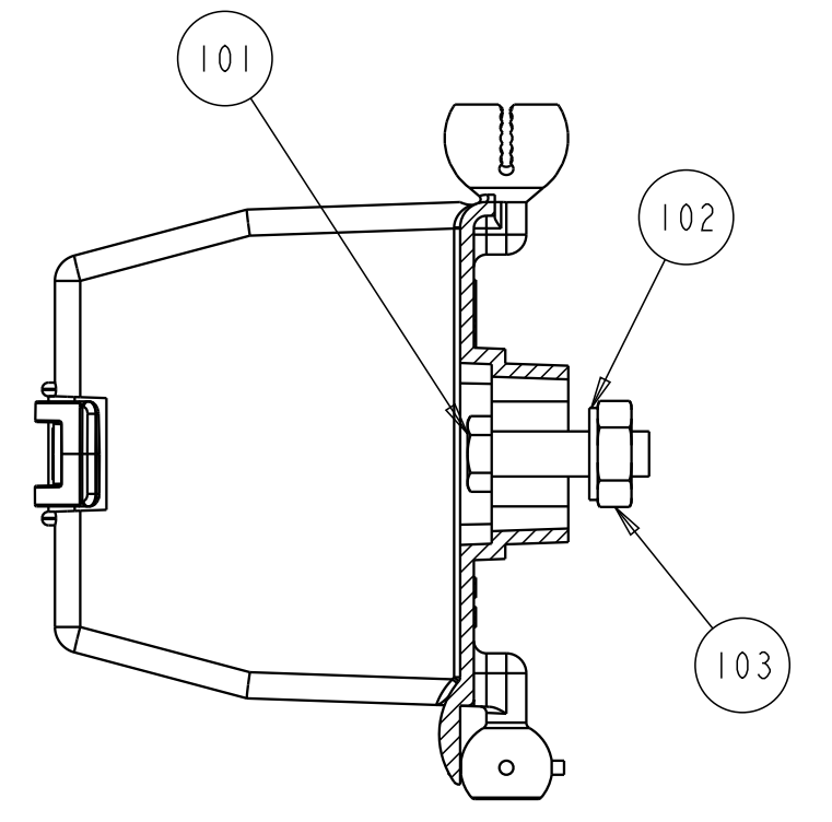
OPTION 2 (IF ATTACHING TO BRACKET WITH CLEARANCE HOLE)
