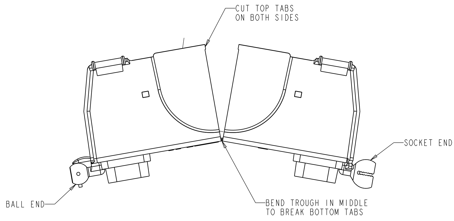
DETAIL A UNIVERSAL TROUGH SPLIT
