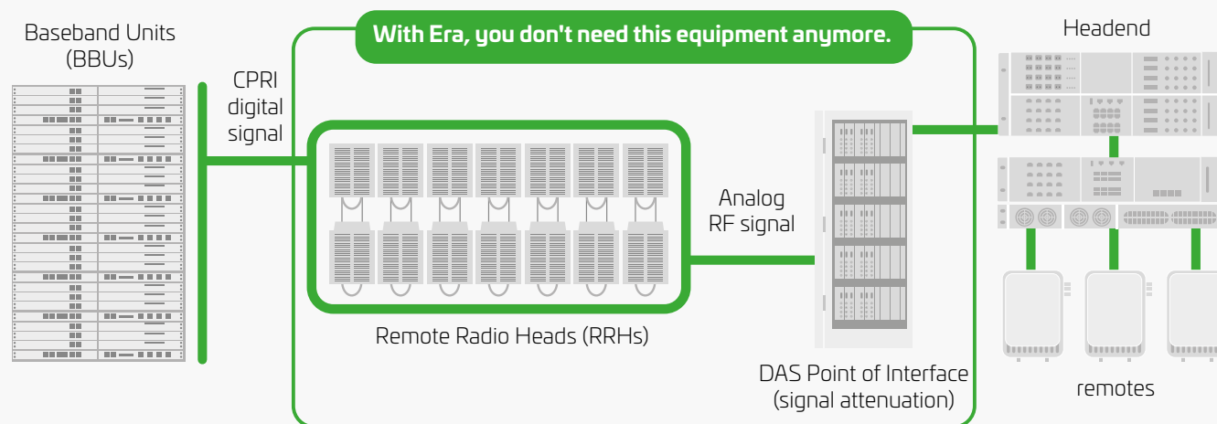
The above figure shows the architecture for a traditional analog DAS system highlighting the remote radio heads (RRHs) in the middle that are eliminated with a digital DAS system. Through a collaboration with Nokia, ERA® features a direct CPRI Digital Donor (CDD) interface to Nokia's AirScale baseband unit (BBU). This integration collapses the functionality of up to six remote radio units and their associated cabling into a single 300 x 145 mm (12 x 6 inch) card. Head-end space and power consumption are drastically reduced while system capacity is increased.
