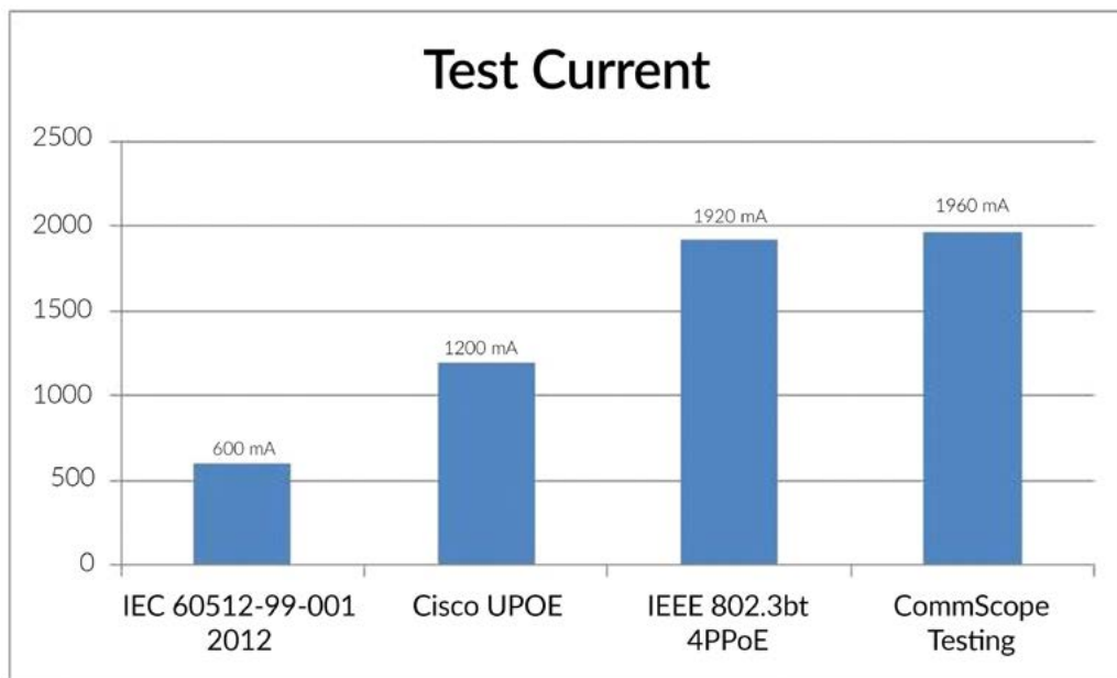
Figure 9: CommScope connector/connecting hardware test current level comparison
