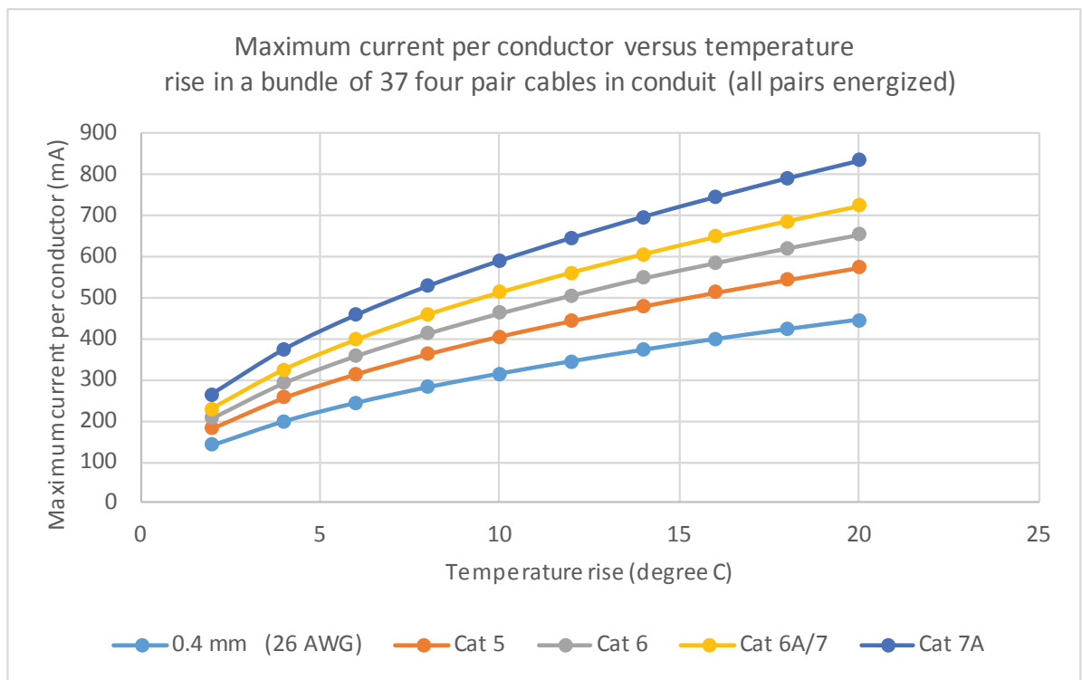
Figure 8: Effects of dc current on cable temperature
