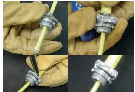
Step 16: Insert the fiber cable into the MC connector and attach to the armor. This will provide protection for the sharp edges of the armor and allow for grounding.
