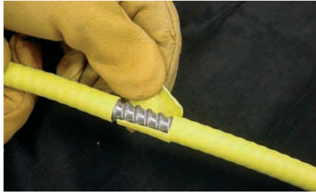
Step 13: Remove outer jacket between ring cuts.
