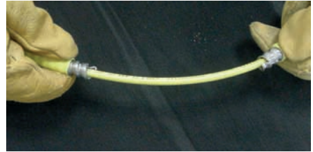
Step 15: Using a twisting motion, separate the armor at the cut and remove the armor from the fiber cable.
