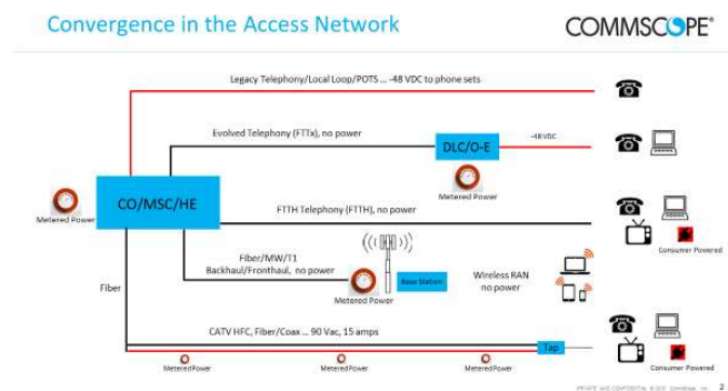
Figure 4 - Convergence in the Access Network
