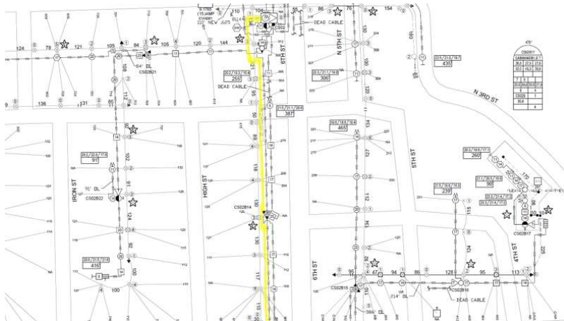
Figure 6 - Fiber and Coaxial overlay in HFC
