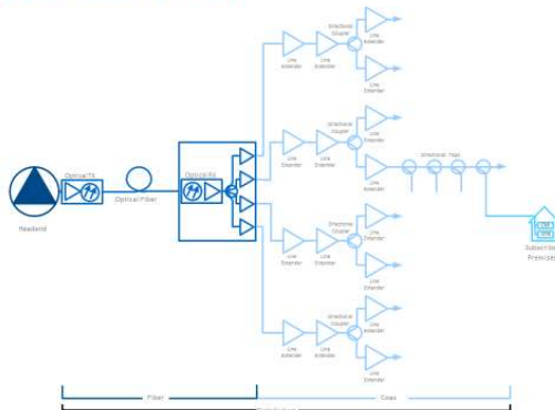
Figure 3 - HFC Network
