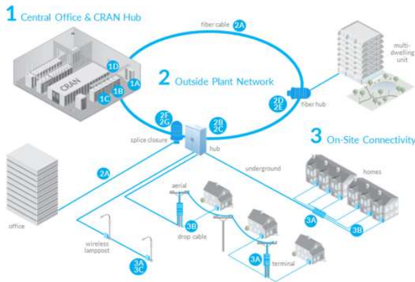
Figure 5 - Network Convergence
