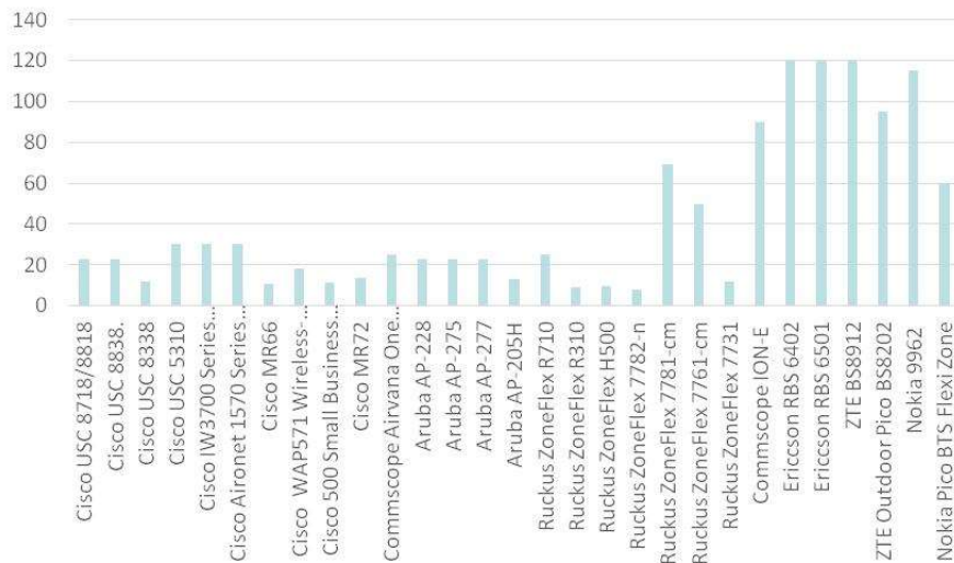
Figure 8 - Access Point Power Requirements
