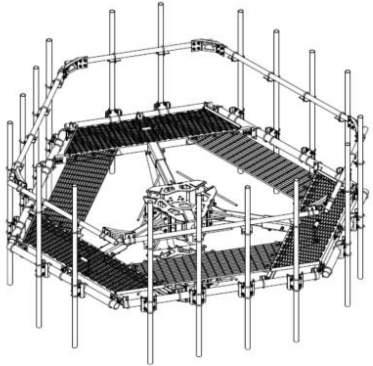
MTC3984 - 6-Sector Monopole Platform
