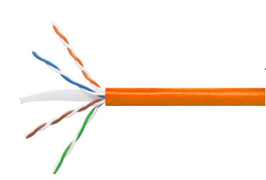
CS34ZB Category 6 U/UTP Cable, low smoke zero halogen, orange jacket, 4 pair count, 305 m length CommPak® box
