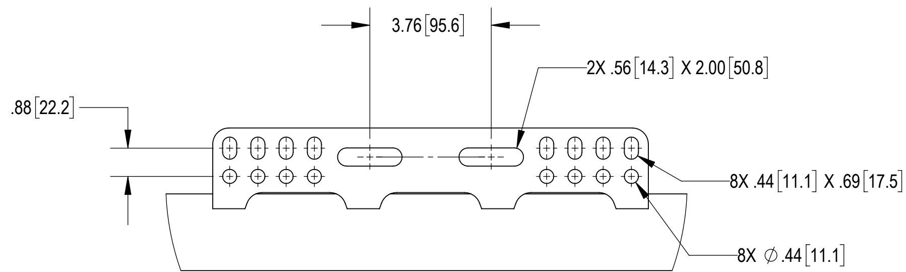
DETAIL E SCALE 1 : 3 2 PLACES
