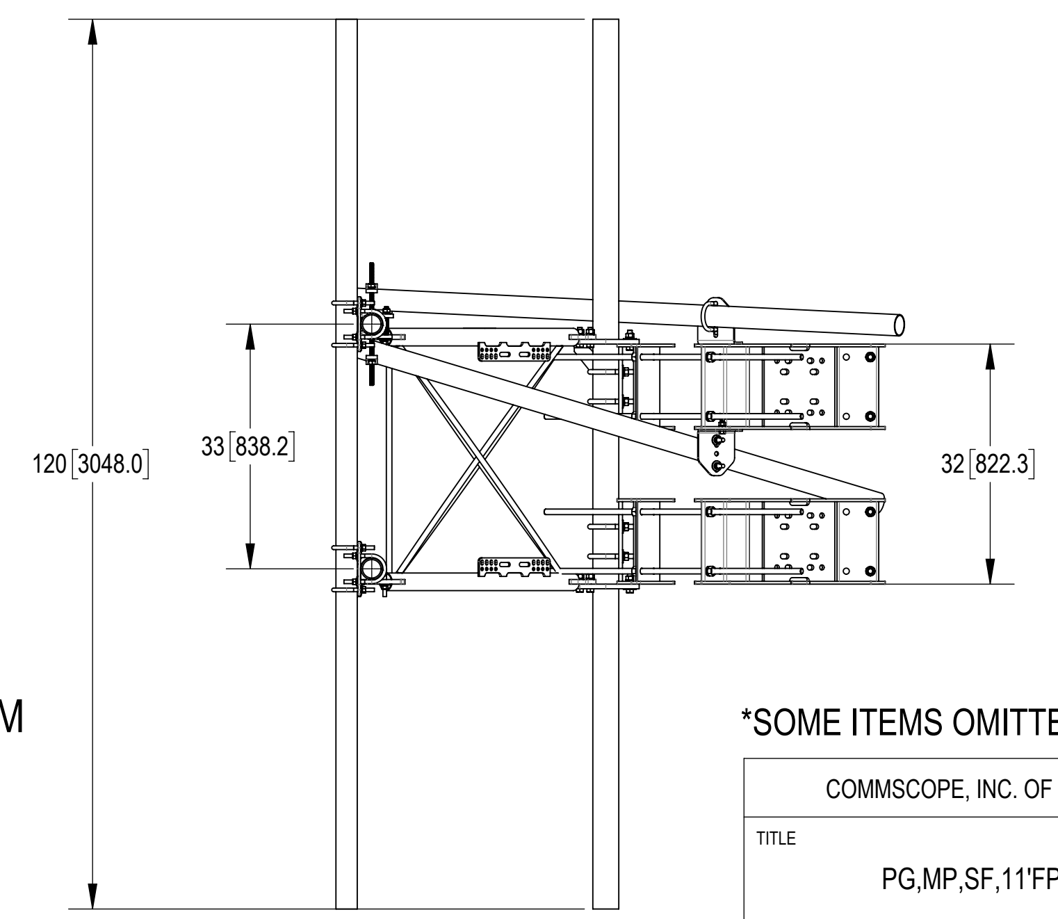
DETAIL D SCALE 1 : 4
