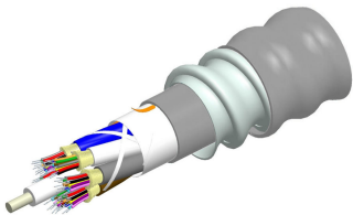
TeraSPEED® Riser Distribution Cable, interlocking aluminum armored with riser jacket, 8 fiber single-unit
