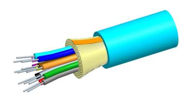
LazrSPEED® Plenum Distribution Cable, 12 fiber single-unit
