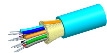
LazrSPEED® Plenum Distribution Cable, 24 fiber single-unit
