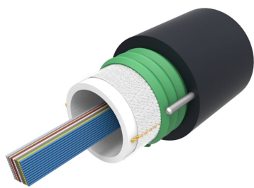
Fiber OSP cable, Steel Armored, Gel-Filled Central Tube Ribbon, 24 fiber, Singlemode G.652.D and G.657.A1, Feet jacket marking, Black jacket color
