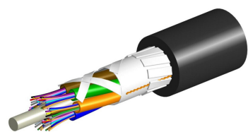
Indoor/Outdoor Fiber Optic Cable, 4-fiber, loose tube, LSZH, OM3, 2000 m
