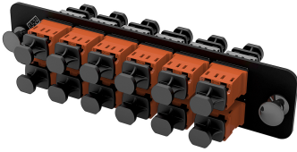
Adapter Pack, Black, 1000-Type, with 12 duplex keyed hybrid LC adapters, orange, no shutter
