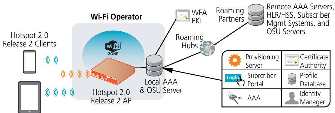
Figure 2: Hotspot 2.0 Release 2 Components
