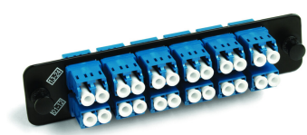
Adapter Pack, Black, 1000-Type, with 12 TeraSPEED® Singlemode duplex LC adapters, blue, no shutter
