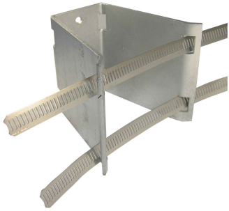
FOSC® Bracket for mounting FOSC 400A or B closure to pole or wall
