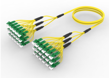
Ultra Low Loss ULL TeraSPEED® LC/APC to LC/APC Ruggedized fanout Cable, 36-Fiber, Plenum, 12 fiber PmP 2.0 mm Dca
