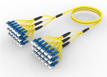
Ultra Low Loss ULL TeraSPEED® LC/UPC to LC/UPC Ruggedized fanout Cable, 36-Fiber, LSZH, 12 fiber PmP 2.0 mm Dca
