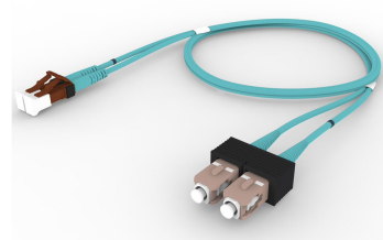
OM4 LC/UPC Keyed Brown to SC/UPC Fiber Patch Cord, 1.6 mm Duplex, Plenum
