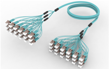
OM4 LC/UPC to LC/UPC 36-Fiber InstaPATCH® 360 Ruggedized Fanout Cable, Low Smoke Zero Halogen
