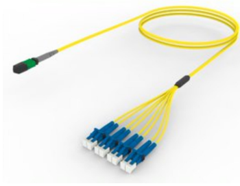
Ultra Low Loss Singlemode MPO8 Pinned to LC/UPC 8-Fiber Plenum Array Cord
