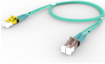
OM4 LC/UPC Keyed Yellow to LC/UPC Fiber Patch Cord, 1.6 mm Duplex, Riser
