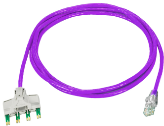
Ultim8 Copper Patch Cord, 4-pair to RJ45, category 6, violet, 10 ft
