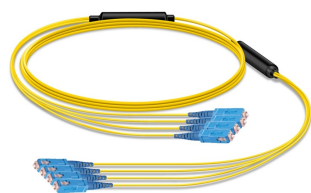
Fiber Optic Patch Cord, Multi-fiber, Singlemode, 4 fibers, SC/UPC to SC /UPC, yellow, 105 m
