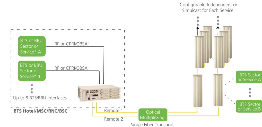
Sample System Configuration
