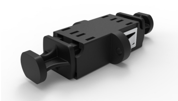
Fiber Optic Insert Adapter, LC, duplex, ceramic sleeve, flanged, multimode, black
