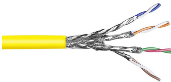
CS67ZC Category 7A S/FTP Cable, low smoke zero halogen, yellow jacket, 4 pair count, 3280 ft (1000 m) length, reel
