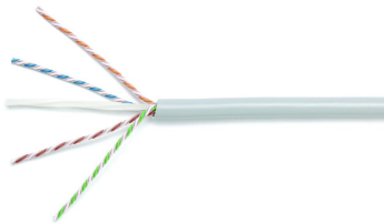
CS44P ETL Verified Category 6A U/UTP Cable, plenum, teal jacket, 4 pair count, 1000 ft (305 m) length CommPak
