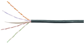
CS34P ETL Verified Category 6 U/UTP Cable, plenum, teal jacket, 4 pair count, 3000 ft (914 m) length, reel
