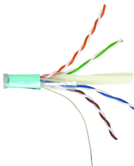
CS44R ETL Verified Category 6A F/UTP Cable, non-plenum, orange jacket, 4 pair count, 1000 ft (305 m) length reel
