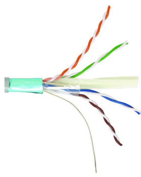
CS44R ETL Verified Category 6A F/UTP Cable, non-plenum, orange jacket, 4 pair count, 3000 ft (914 m) length reel
