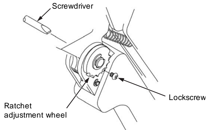
Figure 5. Ratchet Adjustment
