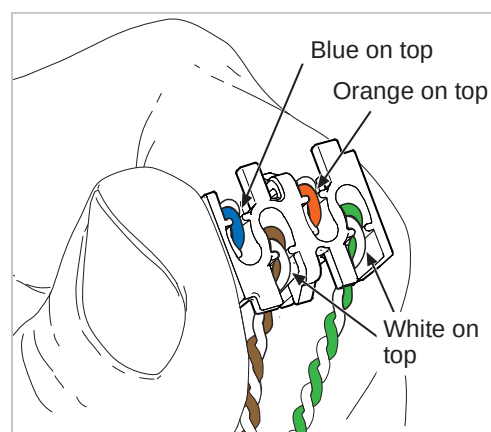
Figure 3. Fold Pairs Back into Slots
