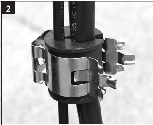
Insert grommet into SnapStak™ hanger.
