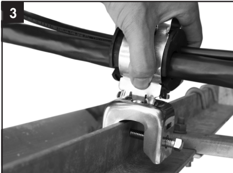
Insert SnapStak hanger into \frac{3}{4} " mounting hole adapter or cable ladder. SnapStak hangers can be stacked 2 high maximum.
