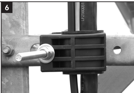
Position block hanger and tighten to tower per hanger installation instructions (3-5Nm).
