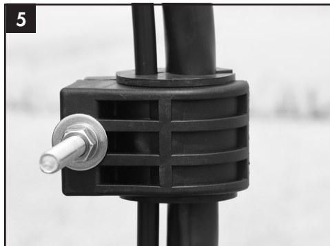
Insert grommet into block hanger.
