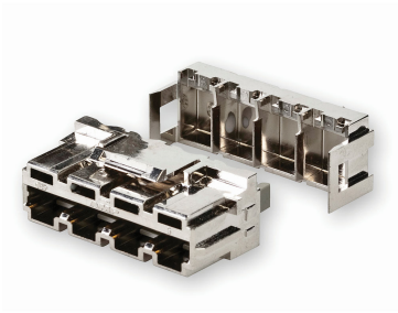
AMP CO Plus Shielded, Edge Connector; Quantity: 100 pieces
