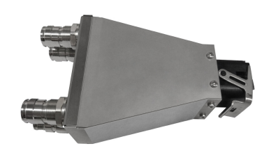
M-LOC Male Multiport Cluster 4 ports to 4.3-10 Female RL Test Adapter
