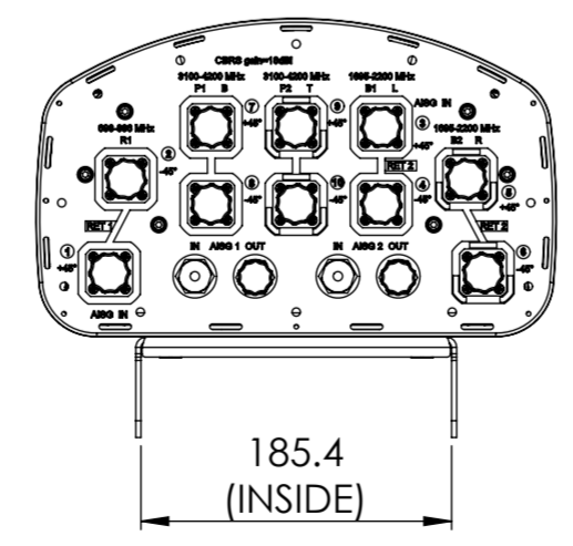
VIEW A-A SCALE 1 : 5
