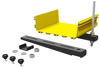
FiberGuide® New Threaded Rod Bracket Kit, 12mm for 4x12in System
