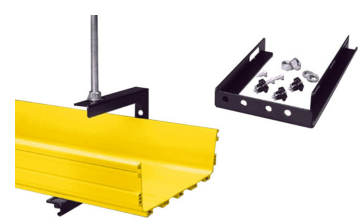
FiberGuide® Low Profile Top Support C-Bracket Kit, 16mm for 4x12in System
