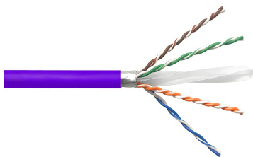
CS41R, ETL Verified Category 6A U/UTP Cable, non-plenum, violet jacket, 4 pair count, 1000 ft (305 m) length reel
