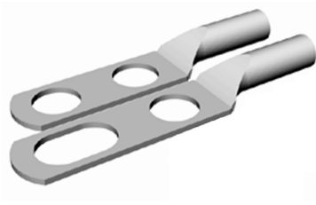
Universal Crimp-on Lug for 3/8 in hardware, #6 AWG, two-hole
