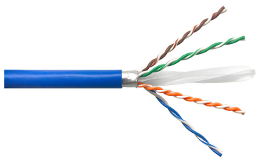
CS41Z1, ETL Verified Category 6A U/UTP Cable, low smoke zero halogen, blue jacket, 4 pair count, 1000 ft (305 m) length reel
