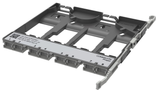
Propel pass-through adapter pack, 8 MPO8-12-24 ports, Type B
