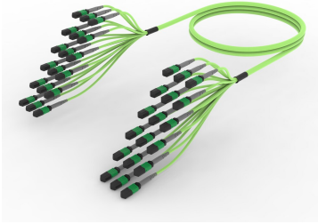
Ultra Low Loss (ULL) OM5 MPO8 APC (Non-Pinned) to MPO8 APC (Pinned), Fiber Trunk Cable Assembly, 144-Fiber, LSZH B2ca
