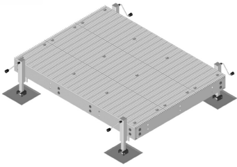
E20® Equipment Platform, 6 ft x 8 ft base with four adjustable legs
