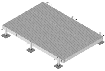
Equipment Platform, 10 ft x 18 ft, base with six adjustable legs
