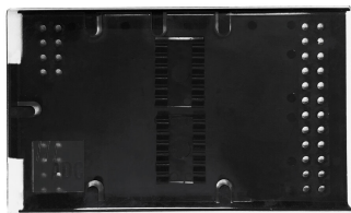
Fiber Optic Splice Tray, 12 splice capacity, heat shrink for FL1 wall box
