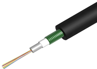
Fiber OSP cable, PE, Gel-filled Central Tube, CST, 12 fiber, Multimode OM4, Meters jacket marking, Black jacket color
